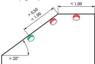
Fig. 19 Straight mounting surface less than 1 m long and 1 m wide
