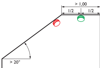
Fig. 18 Straight mounting surface at least 1 m long and 1 m wide
