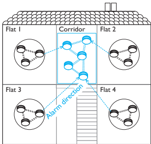
Fig. 21 Example of shared radio group
