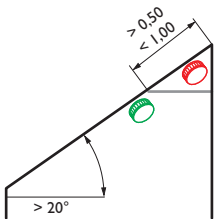
Fig. 17 Rooms with slanted ceilings
