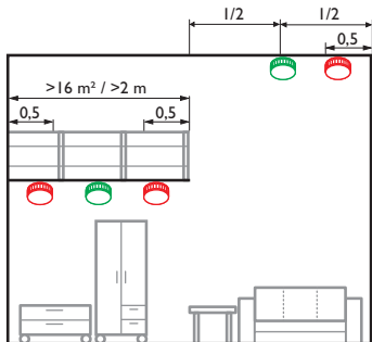
Fig. 20 Rooms with a platform or gallery
